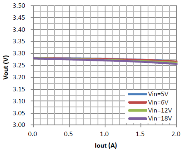
V_{out} vs. I_{out} ( V_{out}=3.3\text{V} )
