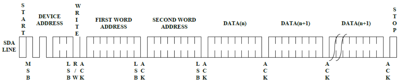
Figure 6. Page Write
