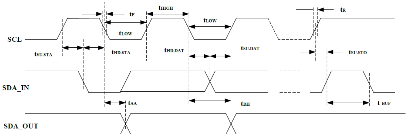
Figure 10. SCL: Serial Clock, SDA: Serial Data I/O
