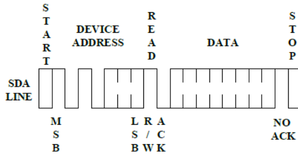
Figure 7. Current Address Read
