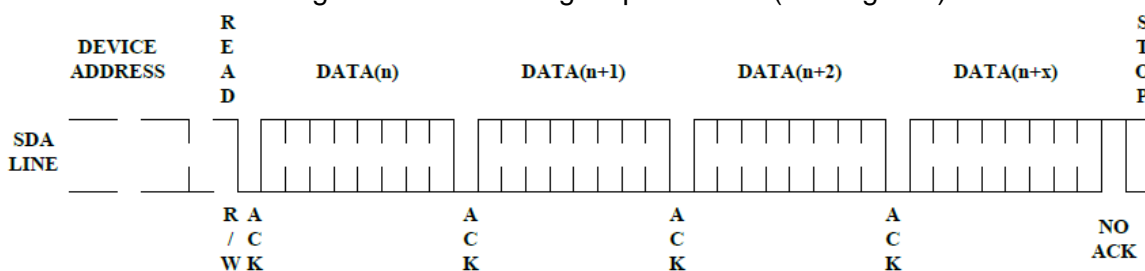
Figure 9. Sequential Read
