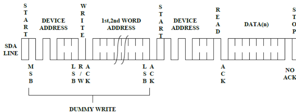
Figure 8. Random Read
