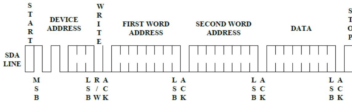
Figure 5. Byte Write
