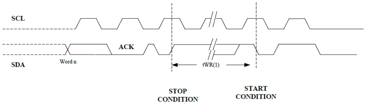
Figure 11. SCL: Serial Clock, SDA: Serial Data I/O
