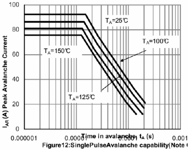
Figure 12: Single Pulse Avalanche capability (Note F)
