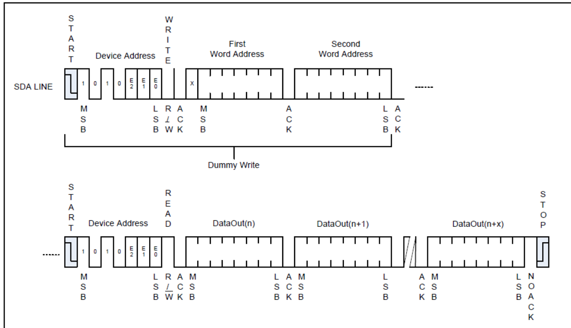
Figure12 : Sequential Read
