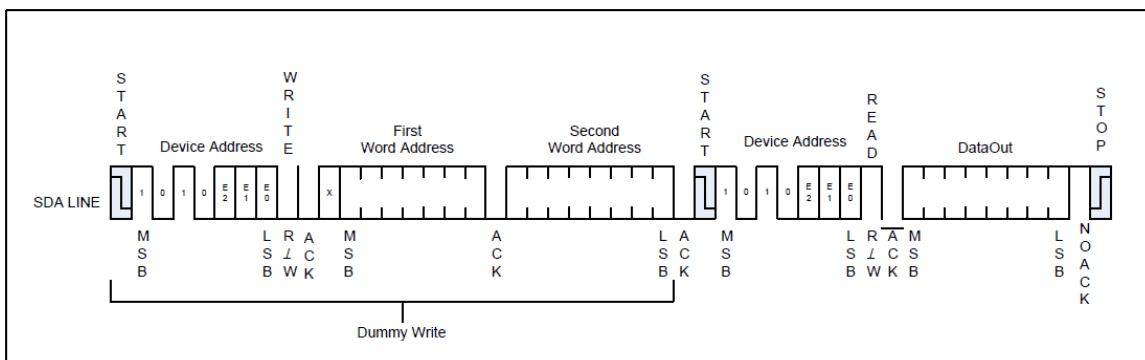
Figure11 : Random Read
